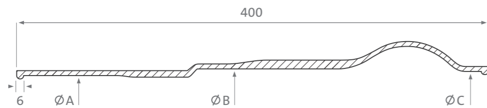
1st Stage Tyre Building Bladder
